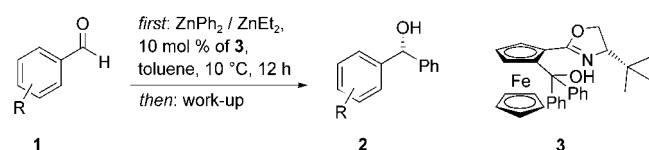
Scheme 1. Phenyl transfer to aromatic aldehydes with a mixture of ZnPh 2 and ZnEt 2 .
